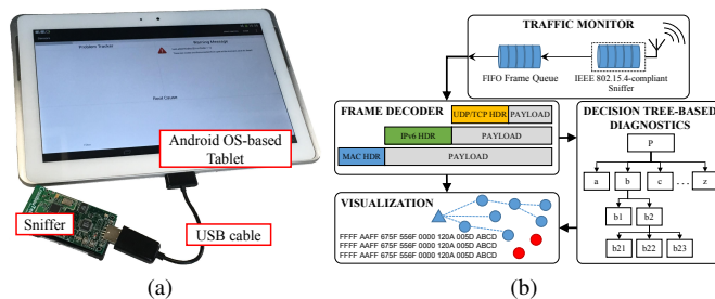
Fig. 3. Handheld diagnostic system: (a) Hardware; (b) Software architecture.
