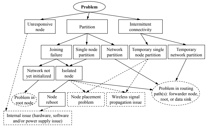
Fig. 2. Simplified decision tree for root cause analysis. Dashed rectangles represent potential root causes that cannot be verified with the current implementation of the system. Dashed ovals represent potential root causes, which cannot be assessed with currently collected network traffic.
