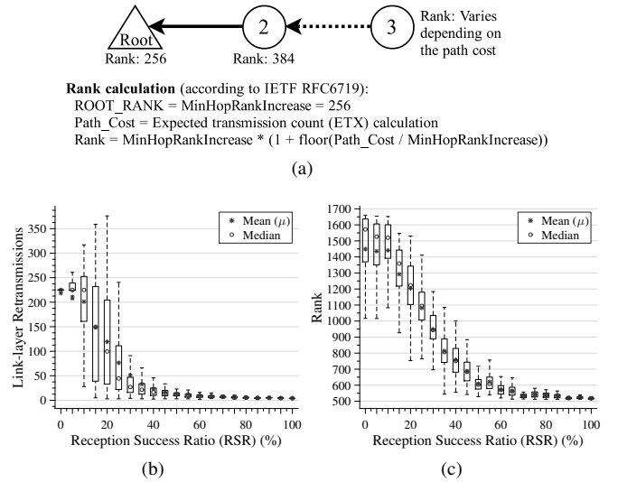
Fig. 4. (a) Three-node linear network simulated in Contiki OS/Cooja. Box plots showing (b) the number of link-layer retransmissions per unicast message (e.g., application data and DAO messages) sent by node 3, and the (c) rank values announced by node 3 through DIO messages. Different reception success ratios (RSRs) for the link between nodes 2 and 3 are considered. Experiments are repeated 10 times.
