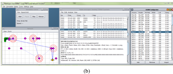
Fig. 5. Deployment at Paddington station box: (a) Model of the site and WSN layout. The figure also shows the average number of connections made by each node to the gateway per day during a 5-day period six months after initial installation [13]; (b) Simulation of Paddington deployment in Contiki/Cooja.
